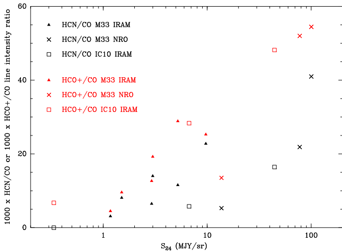
Fig. 9. Link between dense gas fraction and SFR. The HCN/CO and HCO^+/CO ratios are used to trace the fraction of dense molecular gas and the 24 \mu m intensity is used as a proxy for the SFR. HCN/CO is in black and HCO^+/CO is in red. Observations are from Buchbender et al. (2013) and the present work. Typical uncertainties are 20% for HCO^+/CO and 25% for the HCN/CO ratio.
