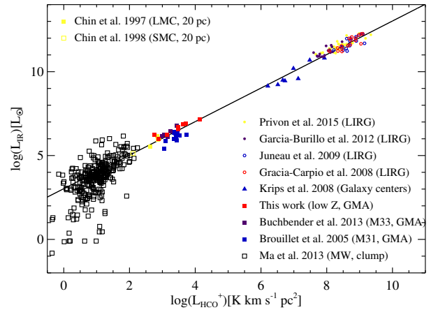
Fig. 10. Link between IR luminosity and HCN (upper panel) and HCO^+ (lower panel) luminosity. The lines show a linear relation between the two quantities. The fits are \log(L_{IR}) = 2.95424 + \log(L_{HCN}) and \log(L_{IR}) = 3.04258 + \log(L_{HCO^+}) and are from respectively Gao & Solomon (2004b) and Graciá-Carpio et al. (2008). The symbols indicate the reference and the scale of the observation.
