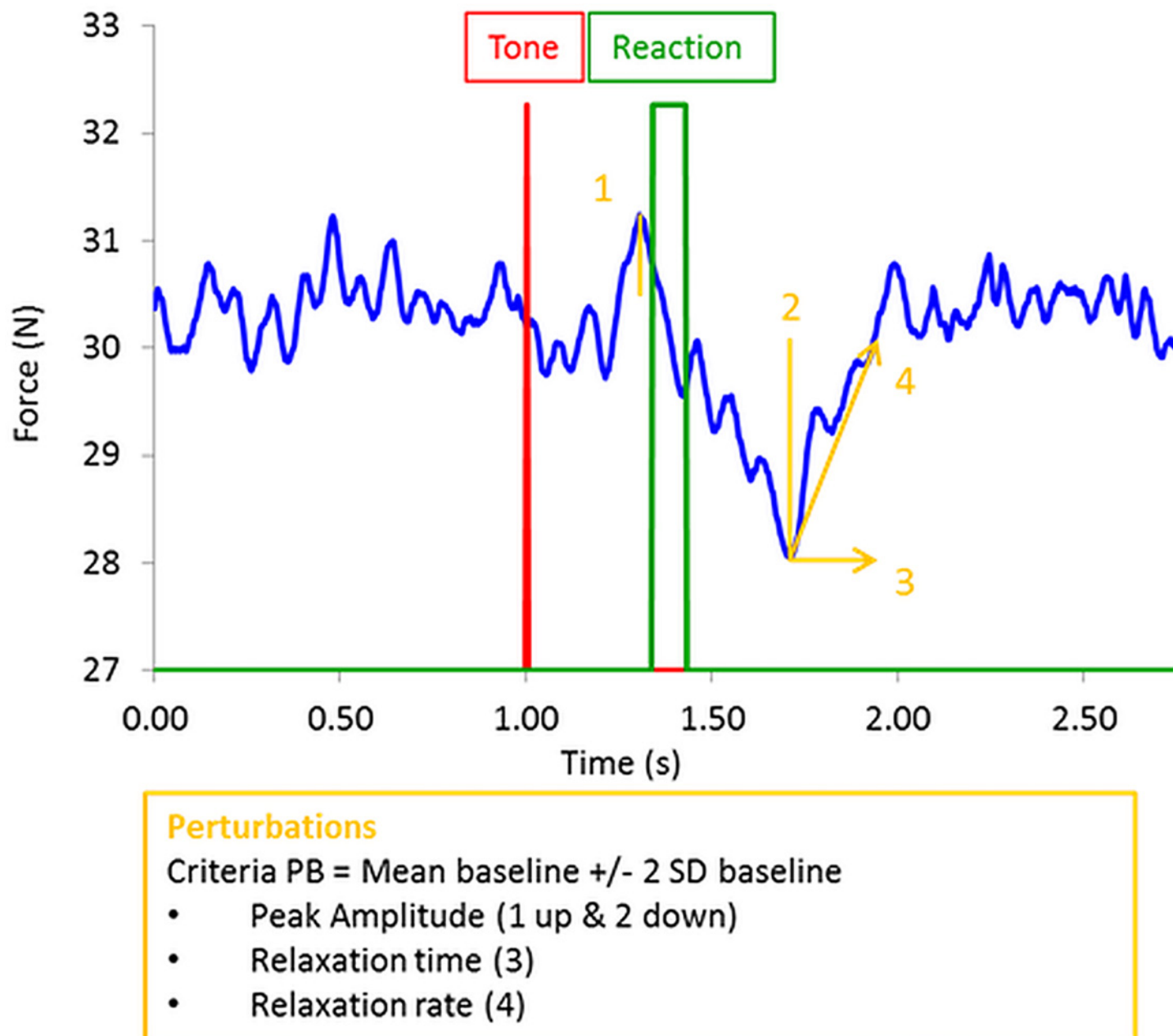
Fig 2. Force-time-series. Representative force-time-series showing a typical perturbation profile. The criterion for the perturbation detection was defined by values crossing the mean of a 1 s baseline before the tone \pm 2 SD of the baseline. Based on this criterion, first, the perturbation upward is detected and expressed in amplitude relative to the prescribed force level; second, the downward perturbation is characterized in the same way. Based on the amplitude and the relaxation time, i.e., the time from the peak amplitude of the downward perturbation till the force reaches the perturbation criteria again, we calculated the rate of relaxation.
