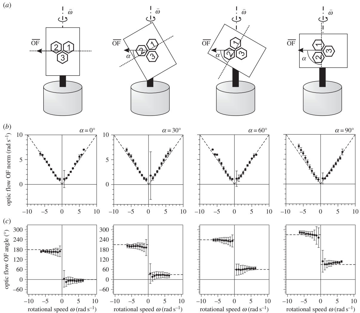
Figure 4. (a) Schematic display of the optic flow characterization set-up, showing the photodetector triplet and optic flow vector \overline{OF} measured during yaw rotational motion at angular velocity \omega for different \alpha roll angles. (b) Optic flow vector norm as a function of yaw rotational speed \omega at four \alpha roll angles. Each data point indicates mean and standard deviation of the OF vector norm computed from signals collected during 30 s at a frame rate of 350 frames s -1 . The dashed line shows the theoretical equivalence between OF norm and rotational speed. (c) Optic flow vector angle with respect to \alpha = 0^\circ as a function of yaw rotational speed \omega at four roll angles \alpha . Each data point indicates mean and standard deviation of OF vector angle values computed from signals collected during 30 s at a frame rate of 350 frames s -1 . The dashed line shows the nominal sensor roll angle \alpha for positive rotational speeds and \alpha + 180^\circ for negative ones.
