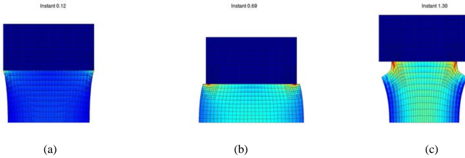
Figure 2: Propagation of damage and creation of a crack within the Arlequin framework (three selected snapshots)
