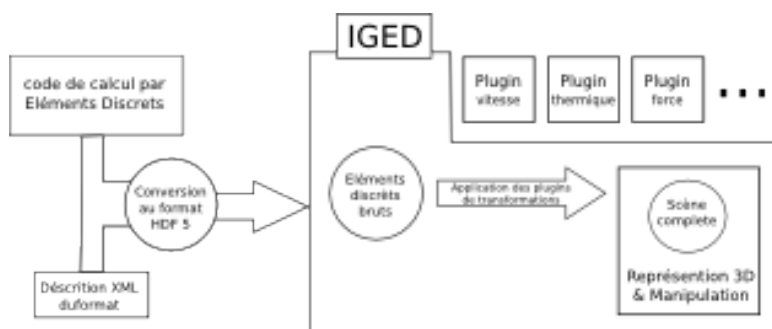
Figure 1 – Architecture de l'Interface Graphique IGED
