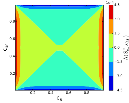
Figure 7: Pairwise invasibility plots for the evolution parameter c going from 0 to 1 with parameters of Table 1 and d = 1.9 .
