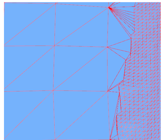
Figure 6: Transition between two DEM with different resolutions.
