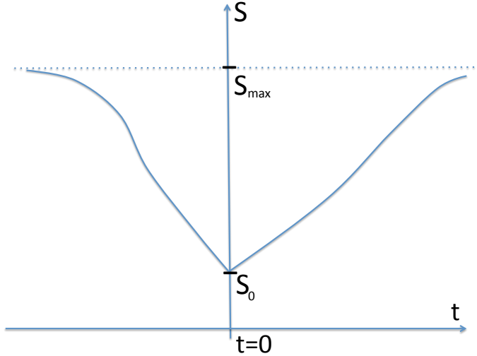
FIGURE 3. Variations of the entropy S .
