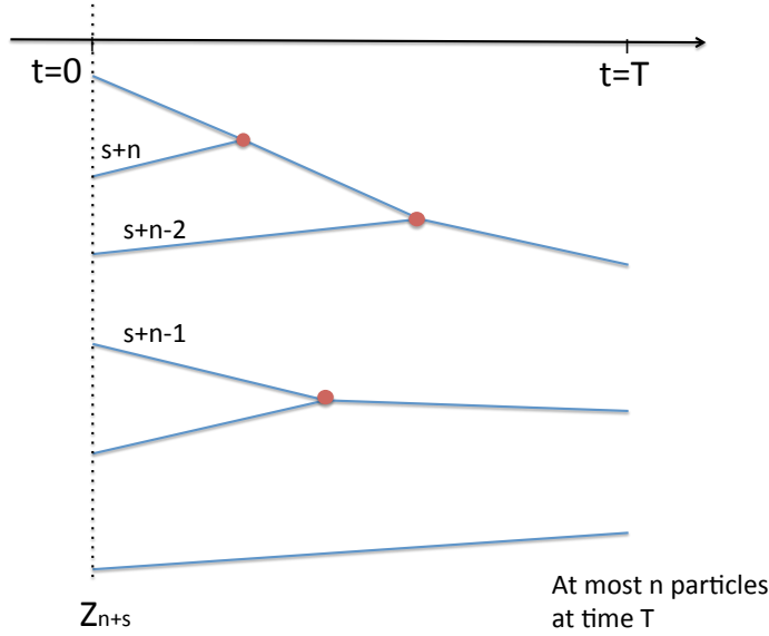
FIGURE 2. Admissible initial configurations.
