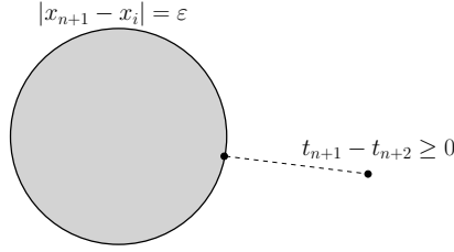
FIGURE 1. The grey domain is an excluded region and its boundary is the surface |x_{n+1} - x_i| = \epsilon corresponding to a collision between particles i and n + 1 . The admissible configurations are outside this domain and can be parametrised by a point of the surface and a non negative time t_{n+1} - t_{n+2} , provided that the velocities are pre-collisional.
