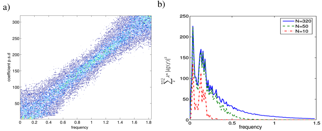
Fig. 22. The frequency is nondimensionalized with the plate thickness a) spectral density of the pressure POD coefficients \hat{a}_p^n b) spectral density of the POD energy \sum_{n=2}^{N+1} \lambda^n |\hat{a}_p^n(f)|^2
