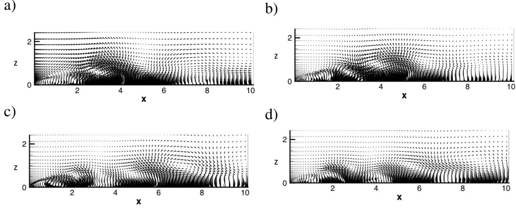
Fig. 24. Pressure-duced spanwise-averaged velocity mode a) n = 2 b) n = 3 c) n = 4 d) n = 5 - the streamwise origin is located at the leading edge of the plate
