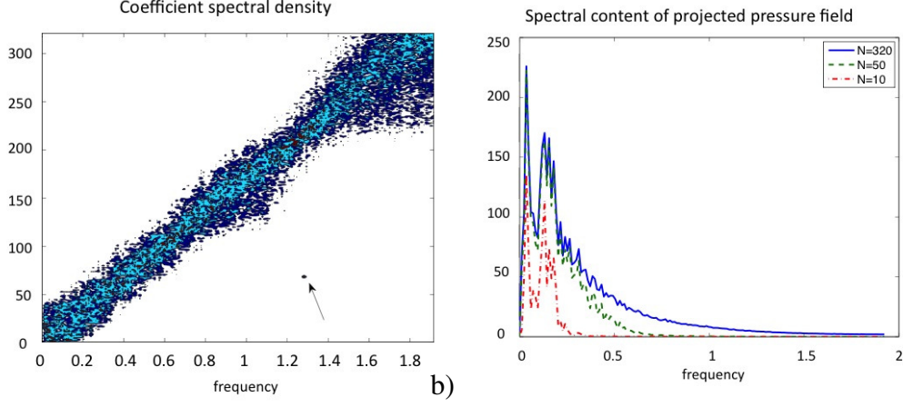
Fig. 18. The frequency is nondimensionalized with the plate thickness a) spectral density of the pressure POD coefficients a_p^n . The arrow indicates the location of the Kelvin-Helmholtz frequency b) spectral density of the POD energy \sum_{n=2}^{N+1} \lambda^n |\hat{a}^n(f)|^2 .
