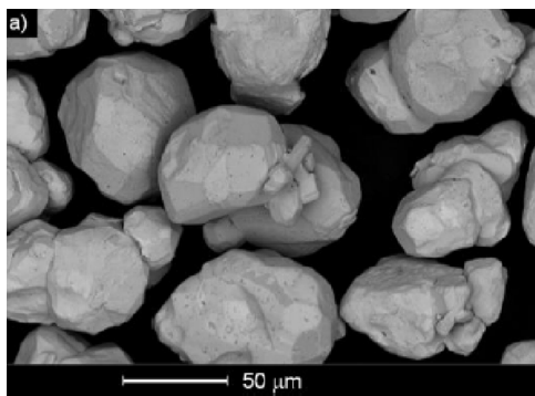
Fig. 6 – SEM view of tungsten particles.
