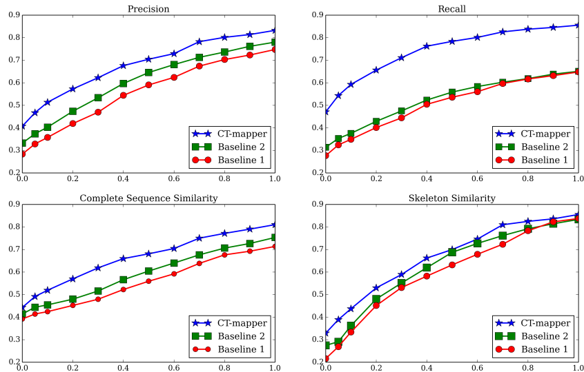
Figure 10: Up-left: Precision, up-right: Recall, bottom-left is Edit-based similarity scores and bottom-right is the skeleton similarity score
