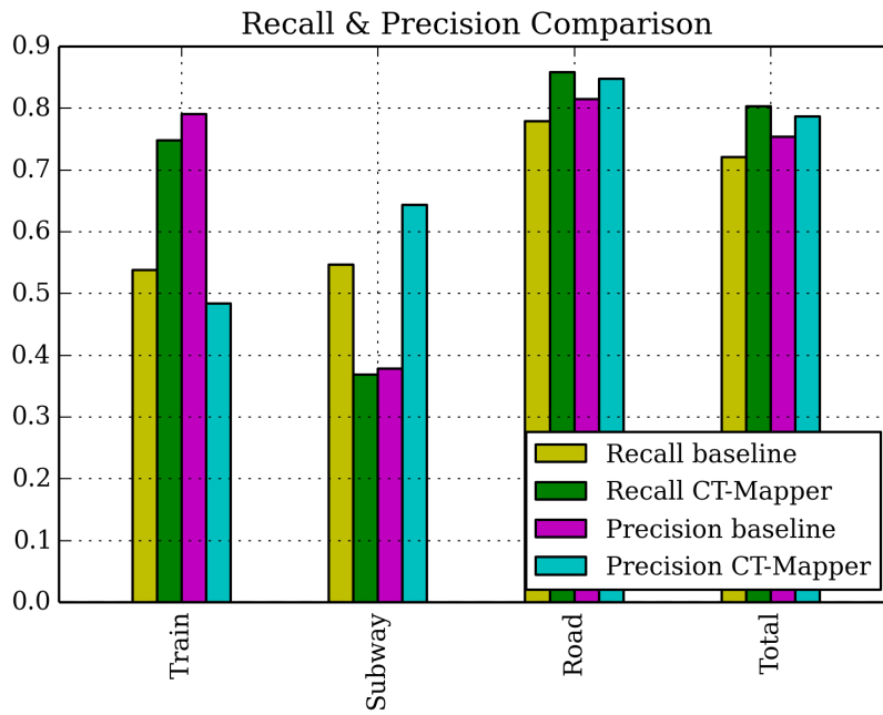
Figure 12: Recall and precision in layer detection
