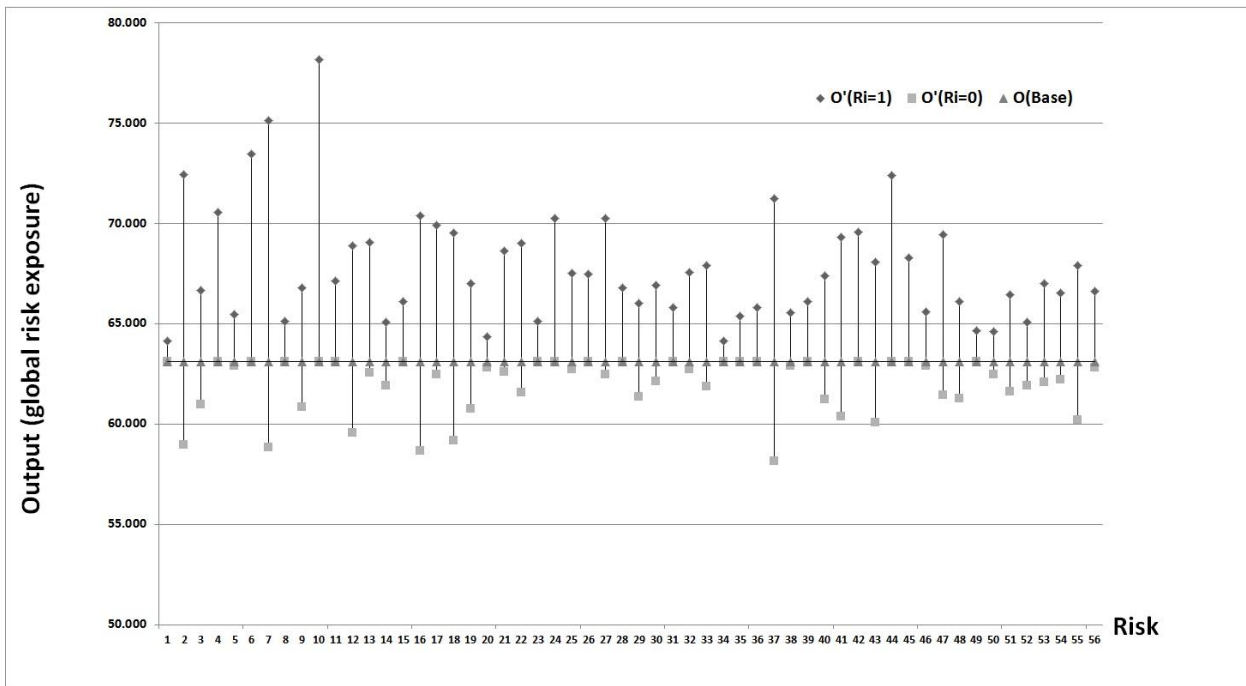
Fig. 3. Illustrating the contribution of each risk on the global risk exposure
