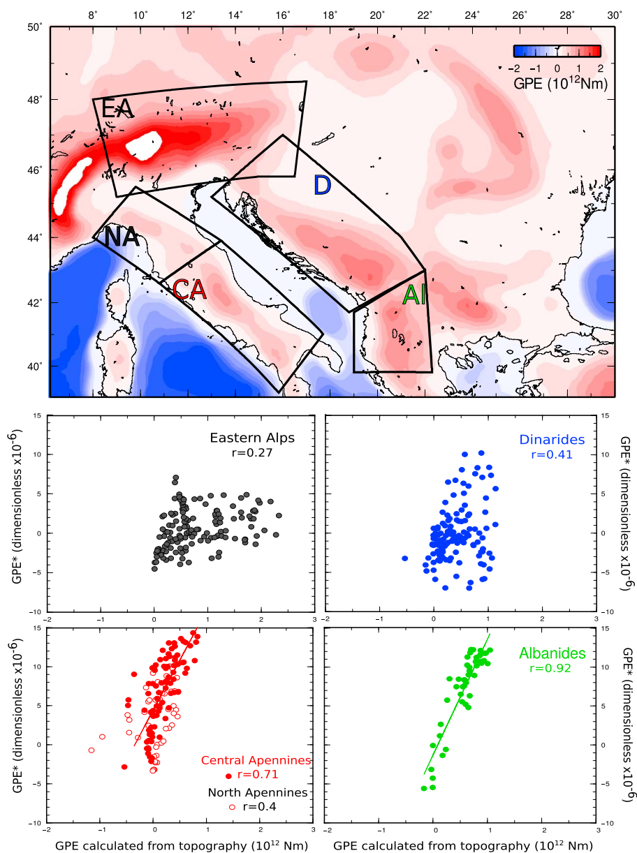
Figure 9. Testing topography control on the peri-Adriatic belts deformation. (top) Map of the GPE calculated from filtered ETOPO1 topography (see equation (7)) assessing Airy isostasy. (bottom) Calculated GPE* from strain, as contoured in Figure 8 against the GPE calculated from topography for several subregions as contoured on the upper map. Least square-estimated best fit linear regressions are plotted as colored lines for Central Apennines and Albanides where the correlation is significant, i.e., where the correlation coefficient r is higher than 0.5.
