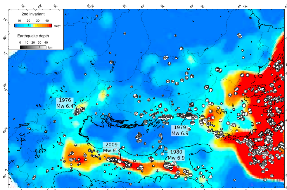
Figure 6. Map of the second invariant of the strain rate tensor over the peri-Adriatic area together with moment tensors of M_w > 4.5 instrumental earthquakes combined from regional Pondrelli et al. [2006, 2011] and global CMT and color coded depending on their epicentral depth. Time and magnitude of the largest instrumental earthquakes are indicated.
