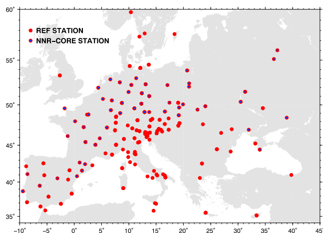
Figure 2. Permanent stations used for reference frame building. Red dots: position of permanent GPS stations used for Eurasia-fixed reference frame building; blue dots: core stations defining its no-net rotation condition.
