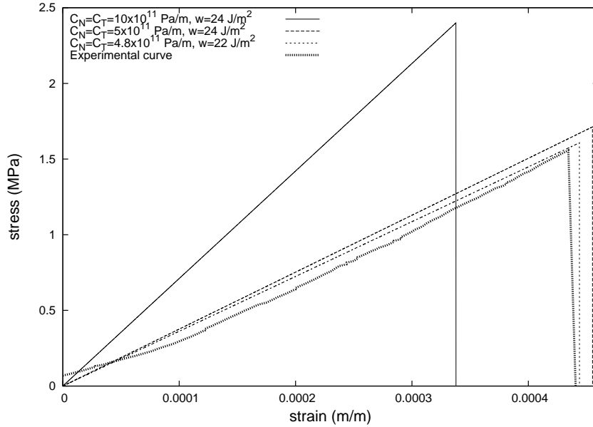
Figure 7: Influence of parameters C_N , C_T and w on the mechanical response
