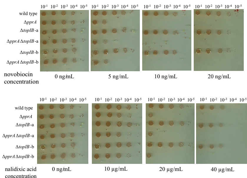
FIG 2 Sensitivity of \Delta pprA mutant to gyrase inhibitors. Serial dilutions of cultures of GY9613 (wild-type), GY14661 ( \Delta pprA ), GY15987 ( \Delta topIB ) (2 clones, a and b), and GY15985 ( \Delta pprA \Delta topIB ) (2 clones, a and b) strains were spotted on plates in the presence or absence of novobiocin or nalidixic acid at the indicated concentrations, and plates were incubated at 30°C for 5 days.
