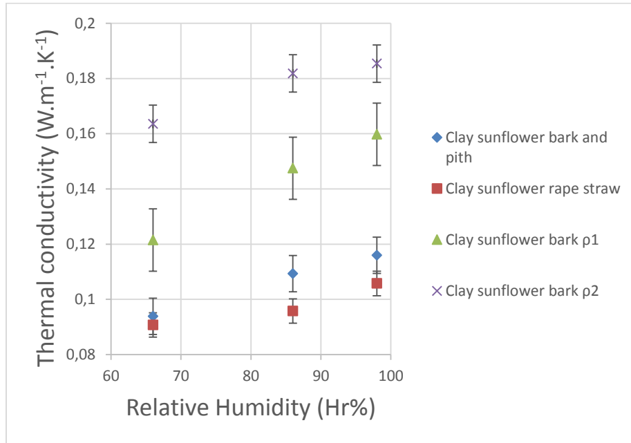
Fig 4. Influence of relative humidity on thermal conductivity for different clay/aggregates' samples
