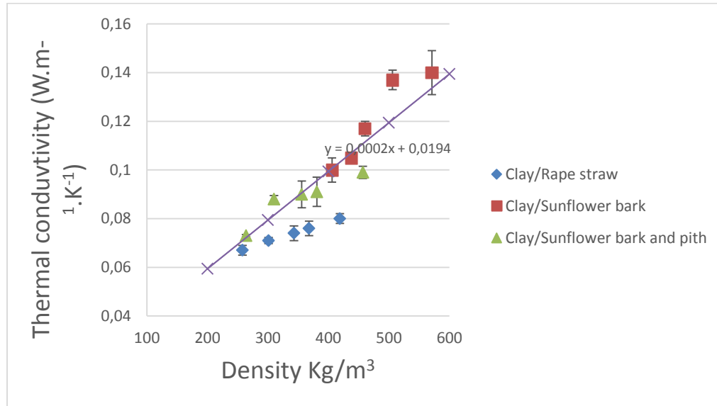
Fig 3. Thermal conductivity versus density of several clay/vegetable aggregates
