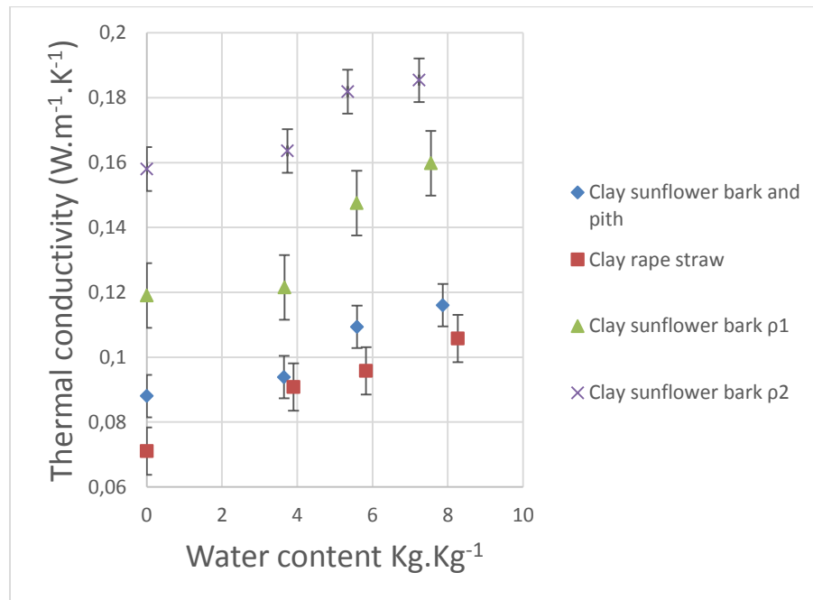
Fig 5. Influence of water content on thermal conductivity for different clay/aggregates' samples
