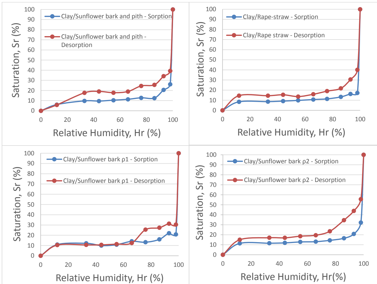
Fig 6. Isothermal sorption-desorption hysteresis of four different mixes of clay/vegetable aggregates' mixes.
