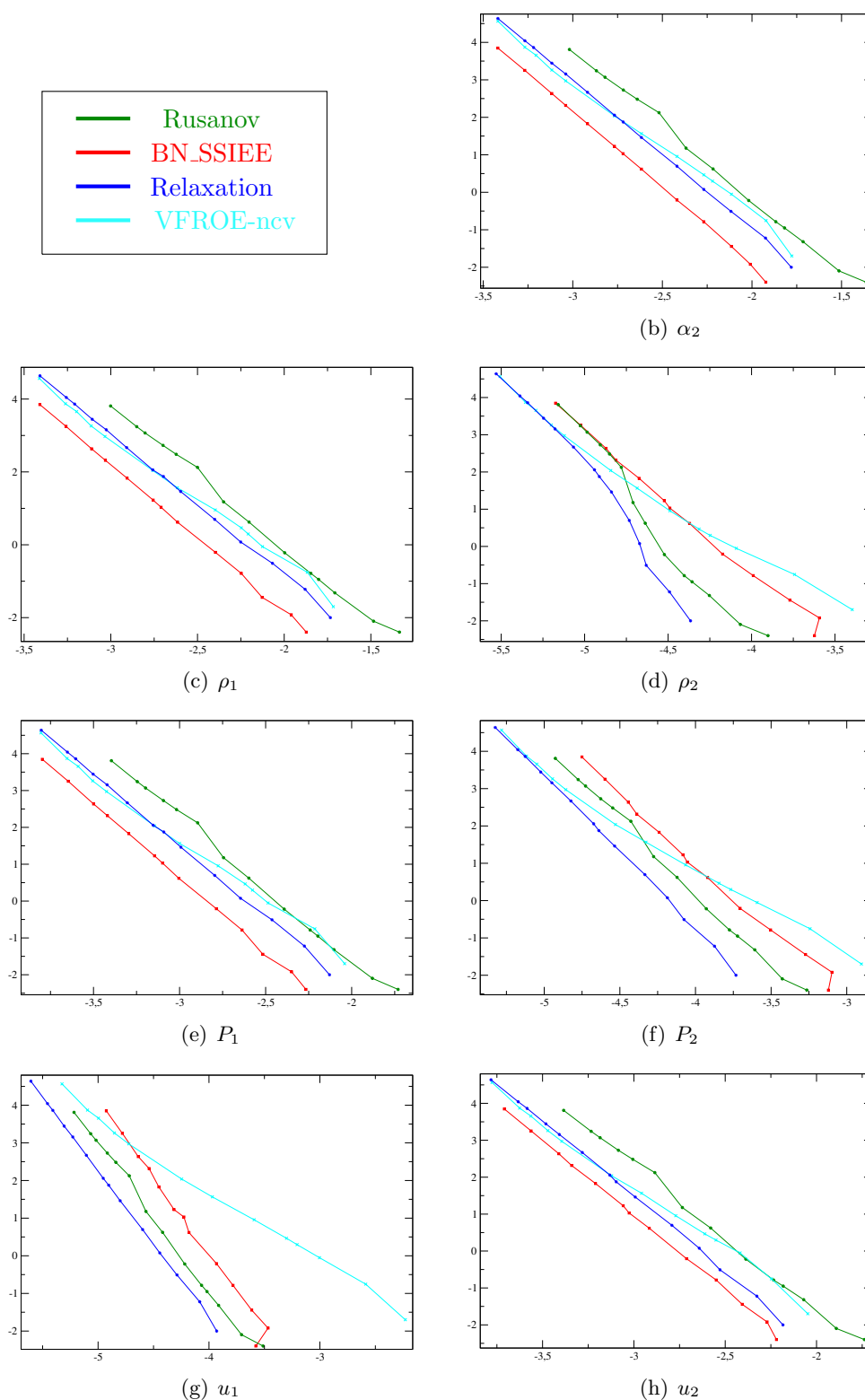
Figure 7: Test 2 - \log_{10} of CPU time as a function of \log_{10} of the error with L^1 norm
