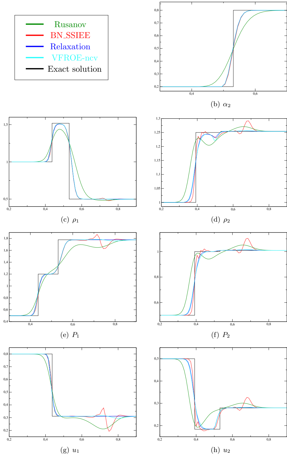
Figure 9: Test 3 - Results with 100 cells
