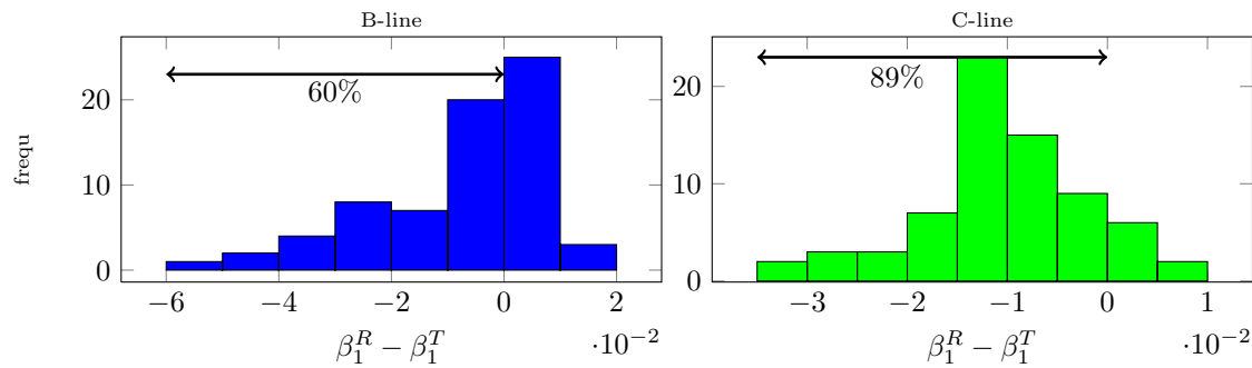
FIGURE 6 Comparison of \beta value in y_1 fit for all NFD-R. For B line and for 60% of days \beta_R < \beta_T . For C line and for 89% of days \beta_R < \beta_T .
