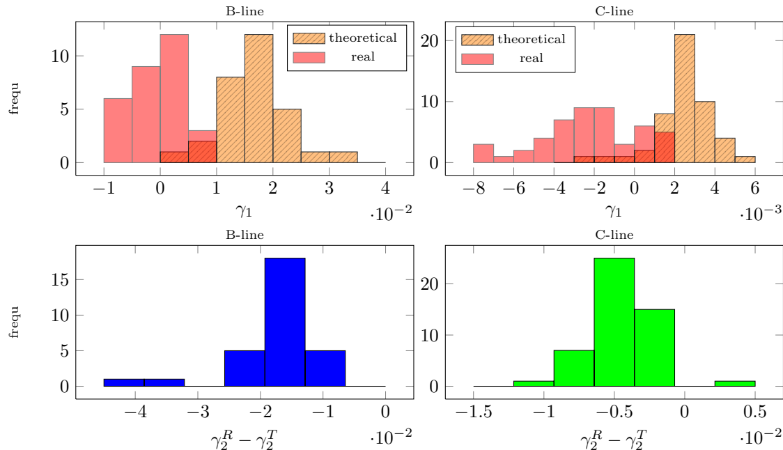
FIGURE 7 Comparison of \gamma value in y_2 fit for filtered NFD-R
