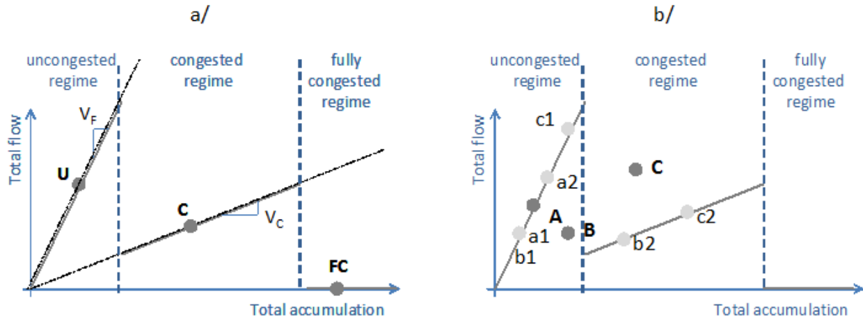
FIGURE 8 local (a) and network (b) theoretical fundamental diagrams of railroad operations in absence of stations. The bold lines of figure a presents the various equilibrium states associated with the train operations blocking rules. Three states are presented; uncongested when trains operates with a free flow speed, congested states, where the speed is strictly limited, and the fully congested points where the trains are stopped. In figure b, three points illustrates the network points associated with two states. Point A is a combination of uncongested states, whereas points B and C are the combination of one uncongested and one congested state.
