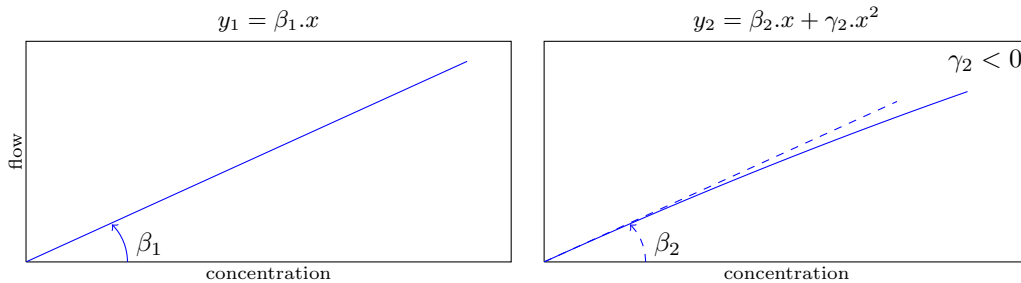
FIGURE 4 The two types of fit; y_1 is a proportional fit where the slope \beta_1 represents an average speed and is expressed in [\text{measure} \cdot \text{min}^{-1} \cdot \text{train}^{-1}] ; y_2 is a quadratic fit where \gamma_2 gives a curvature depending to its sign. A negative \gamma implies a concave curve which means that the average speed decrease when the train concentration increase.
