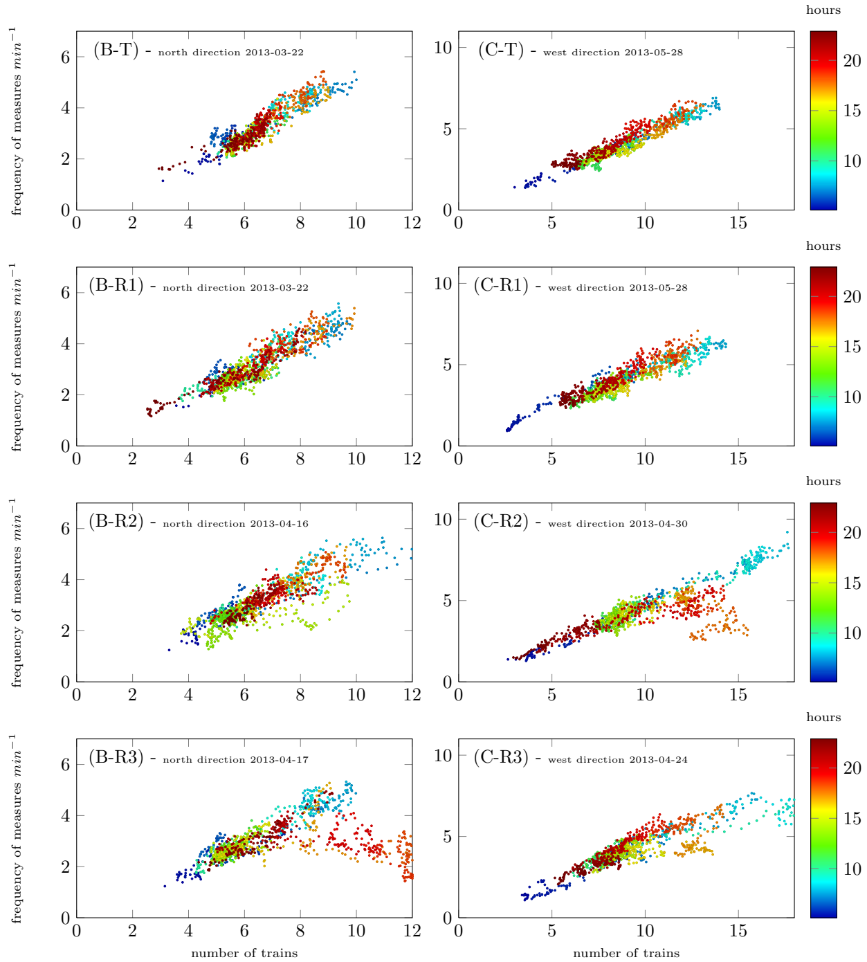
FIGURE 3 examples of NFD-R. (B-T) & (C-T) represent theoretical diagrams, (B-R1), (B-R2), (B-R3), (C-R1), (C-R2) and (C-R3) represent real diagrams.
