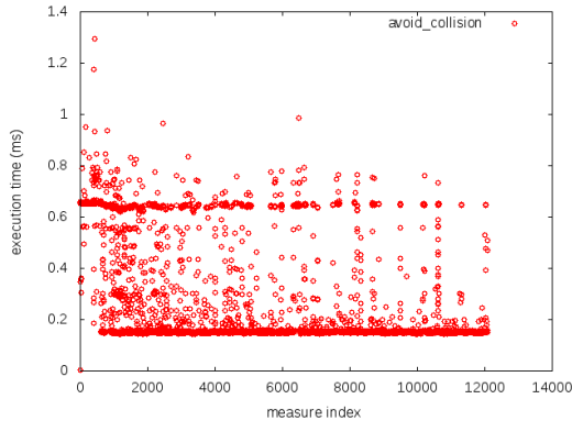
Fig. 3: Execution time measures for codel avoid_collision . Each circle represents a measure.
