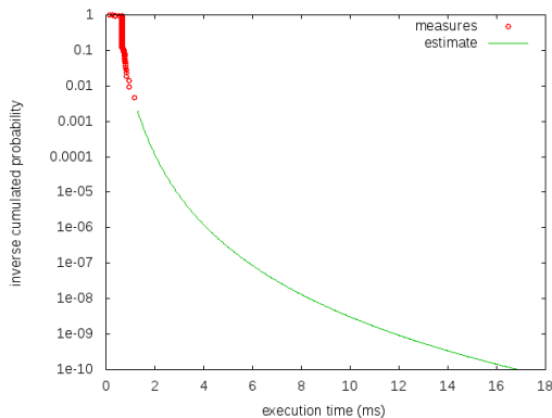
Fig. 4: pWCET estimate for codel avoid_collision
