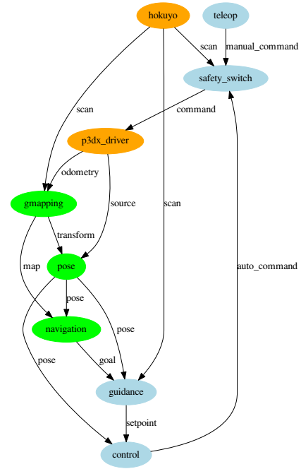
Fig. 2: Navigation component-based architecture. Ovals represent components. Edges represent port connections between components.
