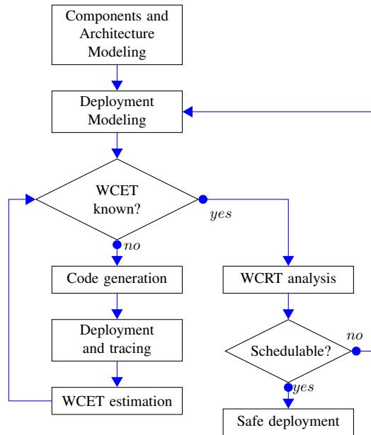
Fig. 1: Real-time analysis process
