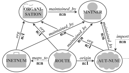
Fig. 2: Entities and relations in the RIPE database relevant for our filter.
