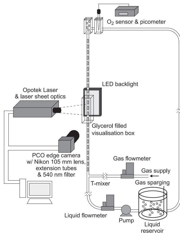
Fig. 2 – Experimental set-up.
