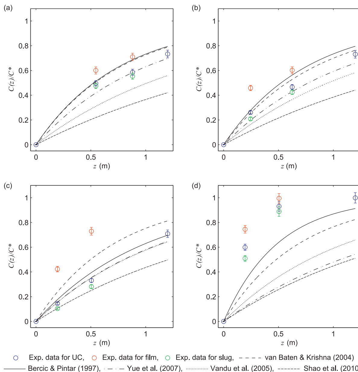
Fig. 6 – Evolution of dissolved O_2 concentration along the channel compared to literature models: (a) Regime 1; (b) Regime 2; (c) Regime 3; (d) Regime 4.
