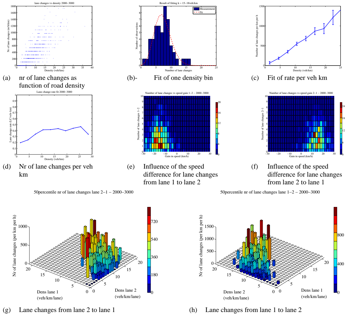
FIGURE 6 The number of lane changes for the part upstream of the off ramp on the A270
