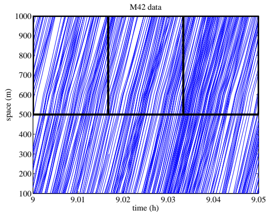
(a) Trajectories of vehicles in all lanes, with , and the black lines denoting the aggregation interval borders.
