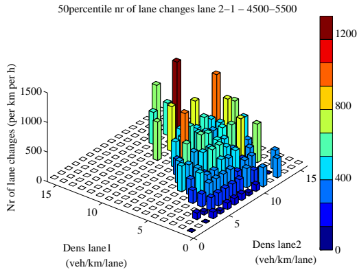
(g) Lane changes from lane 2 to lane 1
