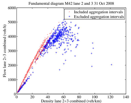
(a) Fundamental diagram in flow-density plane.
