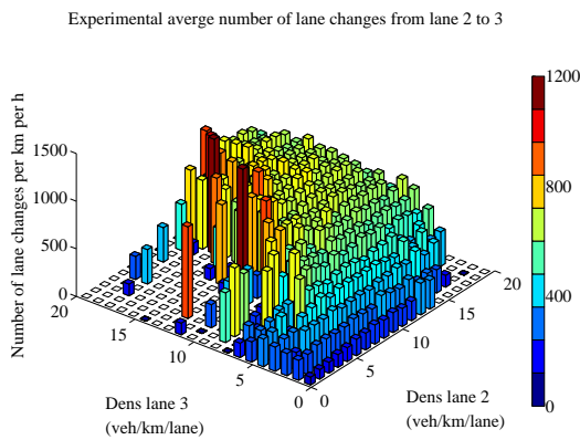
(c) lane 2 to 3
