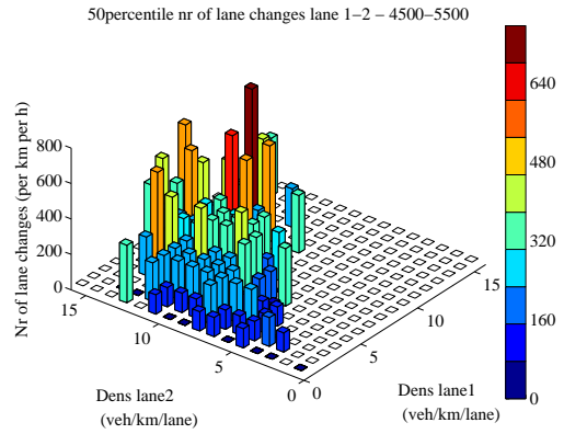
(h) Lane changes from lane 1 to lane 2
