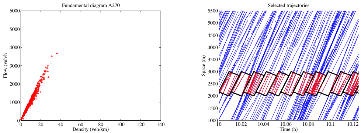
(a) Fundamental diagram
