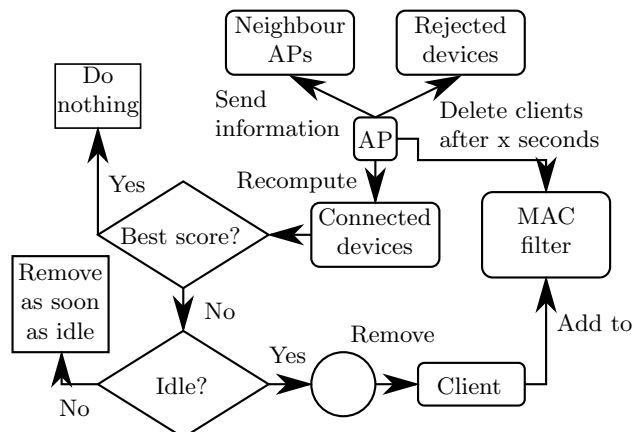
Fig. 3. The AP sends periodic updates to its neighbours and recomputes the score for each connected client.
