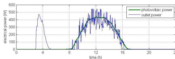
Figure 16. Photovoltaic production and electrical outlets power
