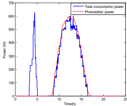
Figure 11. Total power consumption at electrical outlet and photovoltaic power.
