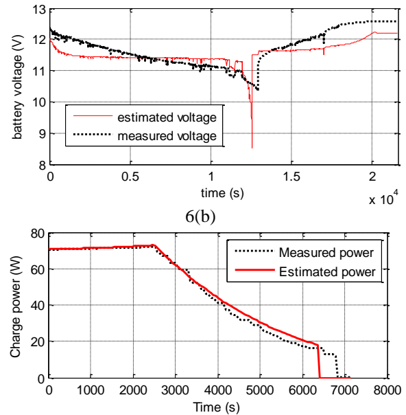
Figure 7. Model validation for power in charge mode.
