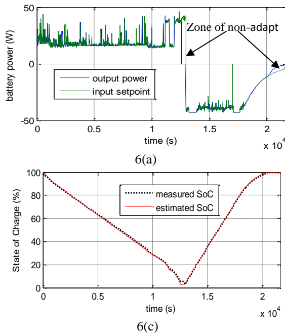
Figure 6. Simulations vs measures for power, voltage and SOC.
