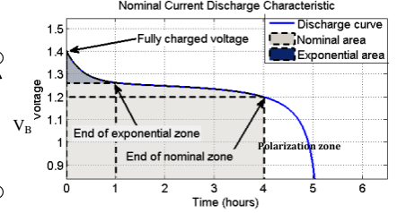
Figure 4. Typical Discharge Curve Characteristics.
