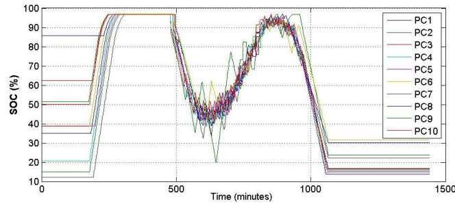
Figure 18. Laptops battery state of charge on real system
