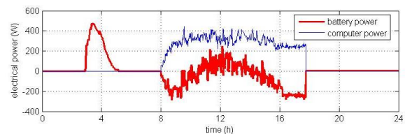
Figure 17. Batteries power (charge and discharge) and computers load.
