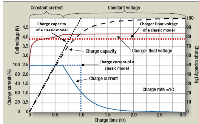
Figure 1. Charge profile of a Li-ion battery
