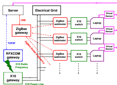
Figure 13. Communication network.
