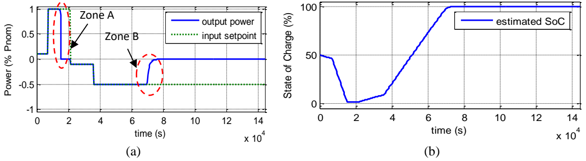
Figure 5. Power and state of charge in different modes.
