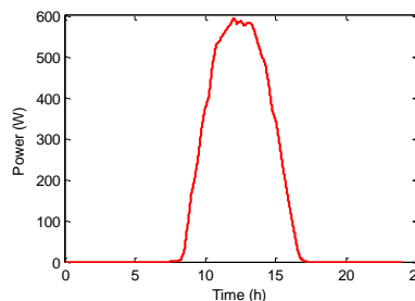
Figure 9. Photovoltaic power.
