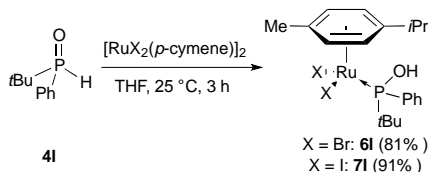
Scheme 2 Synthesis of bromide- and iodide-containing [\text{RuX}_2(\eta^6\text{-}p\text{-cymene})(\text{PA})] complexes.
