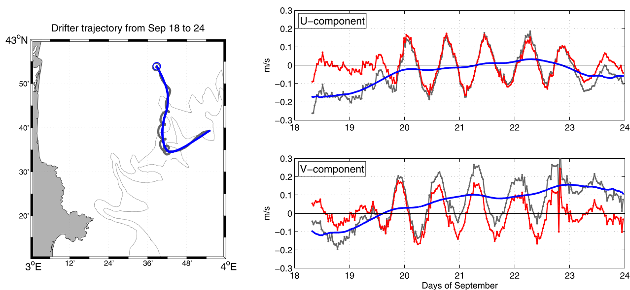
Figure 6. (left) Trajectory of one of the Lyap02 drifters from 18 to 24 September. In gray is the original trajectory, while in blue is the trajectory smoothed with a 17.5 h moving averaging. The larger circle marks the final position of the drifter on 24 September. (right) Time series of the (top) u component and (bottom) v component of velocity obtained by finite differencing the drifter trajectory. In gray are the total velocities \mathbf{u}_{drift} and in blue the 17.5 h moving averaged components \langle \mathbf{u}_{drift} \rangle . The NIO components \mathbf{u}_{NIO} (in red) are obtained as difference between the two.
