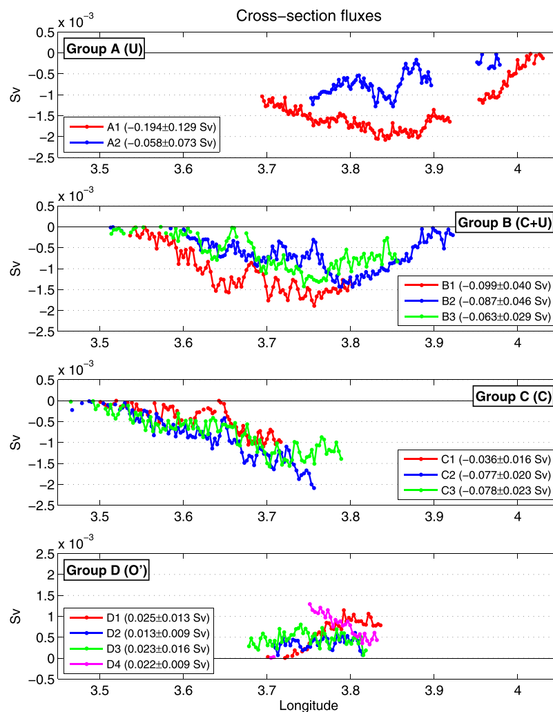
Figure 13. Distribution of the cross-section fluxes ( VT_{tr} , equation (3)) from each individual ADCP measurement along the transects of the four groups from Figure 4. The measurements were corrected for NIO from equation (2) and the associated errors \delta VT_{tr} (equation (A5)) are shown in the legend of each plot. The negative fluxes in the top three plots are associated with outflow of upwelled (U) and/or continental shelf (C) waters from the GoL. The positive fluxes in the bottom plot are associated with inflow of open NW Mediterranean (O') waters. The gap in group A corresponds to a filament of waters characterized by higher SST than U (see Figure 9). Their contribution (a total of 0.023 Sv for transect 1 and 0.008 Sv for transect 2) was therefore excluded from the computation of the total exchanges. Southward waters flowing West of 3.7 with TS characteristics different than U waters were also excluded (total transport of 0.050 Sv for transect 1 and 0.030 Sv for transect 2). For reference, 0.1^\circ in longitude corresponds to a \Delta l of \sim 8.2 km at the GoL latitudes.
