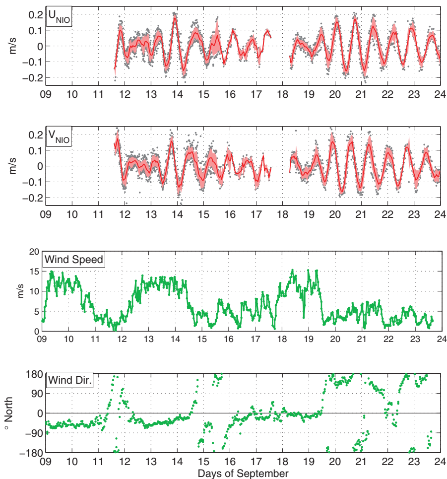
Figure 7. (top) Time series of average NIO velocities ( \mathbf{u}_{NIO} ) (in red) from 9 to 24 September. The velocities were computed by hourly averaging the NIO velocities \mathbf{u}_{NIO} (gray dots) derived from all the available drifters. The red-filled contour marks the one standard deviation confidence interval \langle \mathbf{u}_{NIO} \rangle \pm \sigma_{NIO} . The two gaps from 9 to 11 September and from 17 to 18 September correspond to periods when no drifters were operative in the western GoL. (bottom) Time series of the 30 min averaged wind speed and direction recorded from the R/V Le Suroit for the same period.
