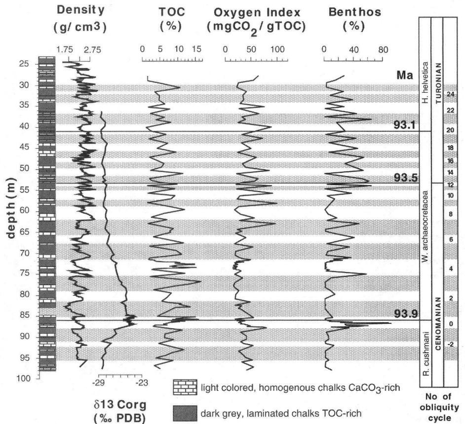
Fig. 3. Cyclostratigraphy and the global late Cenomanian \delta^{13}C_{org} excursion in exploration well S75 of the Tarfaya-Laayoune Basin. Numbered cycles correspond to 39 kyr obliquity cycles (data from Kuhnt et al., 1997 and Luderer and Kuhnt, 1997). Original color image appears at the back of this volume.
