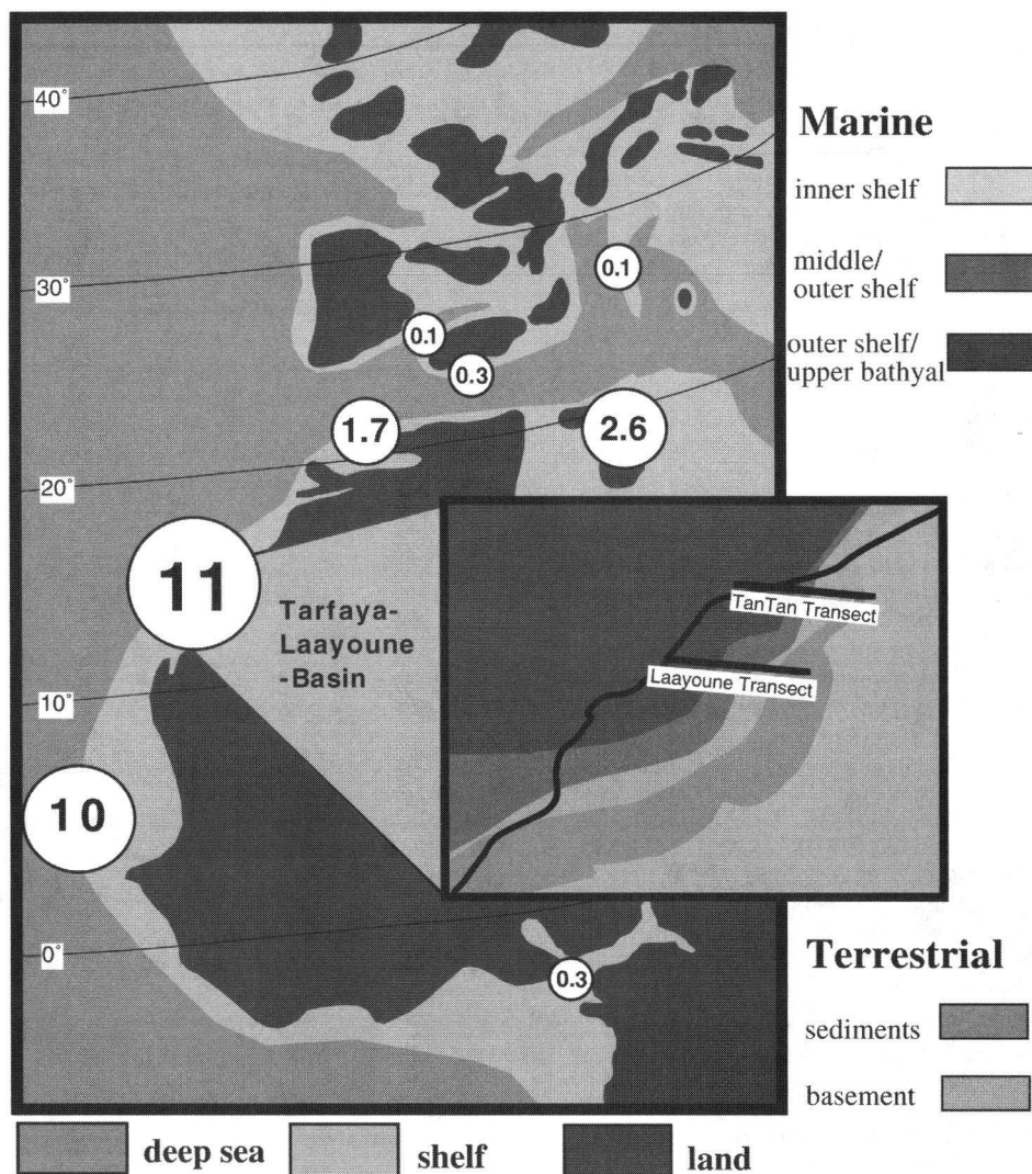
Fig. 1. Turonian paleogeography of the Tarfaya-Laayoune Basin [modified from Kuhnt et al., 1990]. Values in circles are organic matter accumulation rates during the Cenomanian/Turonian oceanic anoxic event (OAE) 2 (in grams per square meter and year). Original color image appears at the back of this volume.
