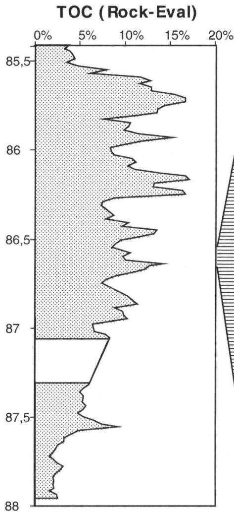
Fig. 4. Nested cycles in TOC-content of 3–4 kyr frequency (obliquity cycle 0, late Cenomanian, well S75) and millimeter-to-centimeter-scale cyclicity (decadal) within the laminated blackshale (polished rock-slab, well S13, Whiteinella archaeocretacea foraminiferal zone; height of the slab is 8 cm). Original color image appears at the back of this volume.
