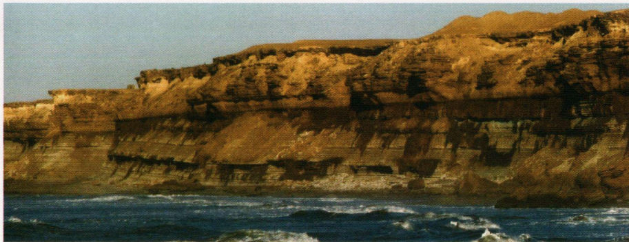
Fig. 2. Cenomanian sediments exposed along a continuous 20-km-long transect reflecting transition from marginal marine to outer shelf paleoenvironments ("Mohammed Plage" coastal section southwest of the mouth of the Chebeika River between Tarfaya and TanTan; the height of the cliff is 30 m).
