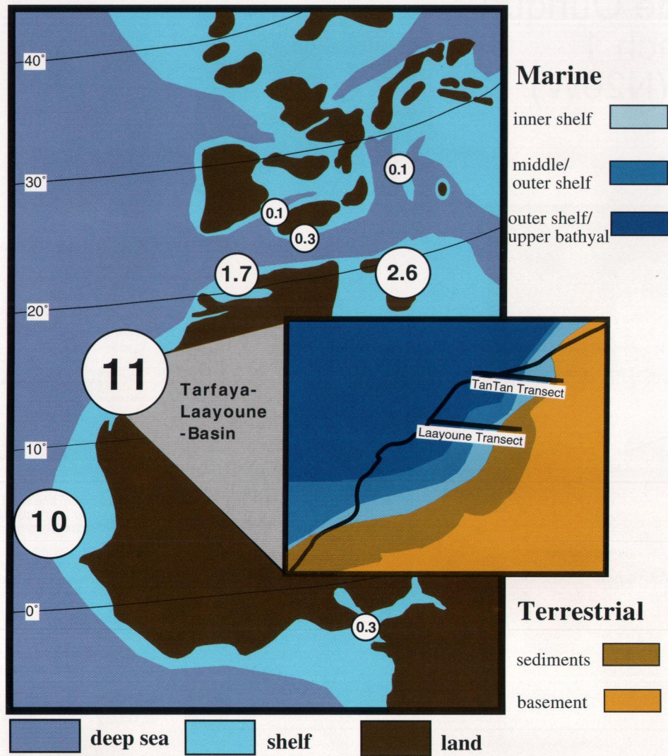
Fig. 1. Turonian paleogeography of the Tarfaya-Laayoune Basin [modified from Kuhnt et al., 1990]. Values in circles are organic matter accumulation rates during the Cenomanian/Turonian oceanic anoxic event (OAE) 2 (in grams per square meter and year).
