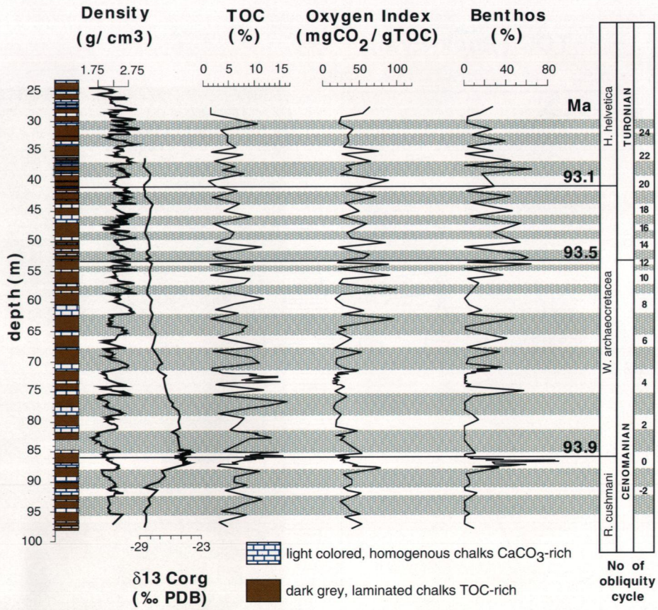
Fig. 3. Cyclostratigraphy and the global late Cenomanian \delta^{13}\text{C}_{\text{org}} excursion in exploration well S75 of the Tartaya-Laayoune Basin. Numbered cycles correspond to 39 ky obliquity cycles (data from Kuhnt et al., 1997 and Luderer and Kuhnt, 1997).
