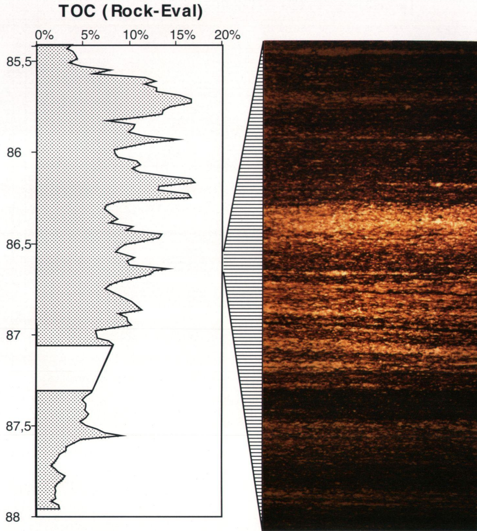
Fig. 4. Nested cycles in TOC-content of 3–4 kyr frequency (obliquity cycle 0, late Cenomanian, well S75) and millimeter-to-centimeter-scale cyclicality (decadal) within the laminated blackshale (polished rock-slab, well S13, Whiteinella archaeocretacea foraminiferal zone; height of the slab is 8 cm).
