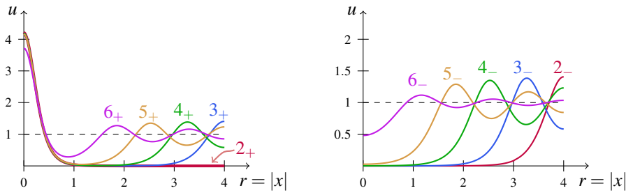
FIGURE 19. Non constant radial solutions ( N = 3, p = 3, R = 4, \epsilon = 0.05 ).
