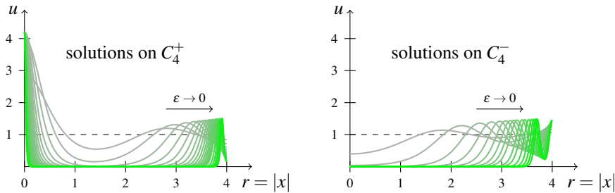
FIGURE 20. Profile of the solutions along the branch emanating from \epsilon_4 ( N = 3, p = 3, R = 4 ).
