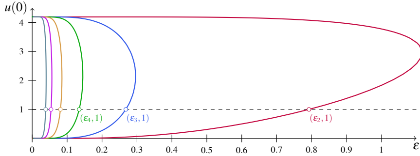
FIGURE 18. Some radial bifurcation branches emanating from (\epsilon_i, 1) ( N = 3, p = 3, R = 4 ).
