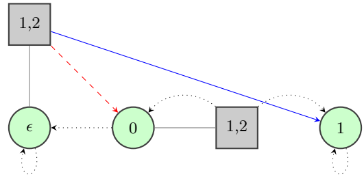
Figure 2: States are indicated by circles, with the reward at each state written within. Squares indicate action pairs at each state. Black dotted lines indicate agreement in the transition, while solid blue lines the model of player 1, and red dashed ones that of player 2.
