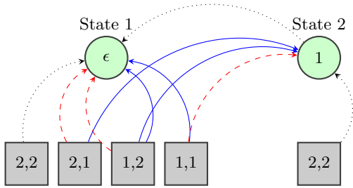
Figure 1: Non-dominating counter-example. States are indicated by circles, with their reward written within. Squares indicate action pairs at each state. Black dotted lines indicate agreement in the model, while solid blue lines the model of player 1, and red dashed ones that of player 2. Omitted action pairs have arcs directly from the state.
