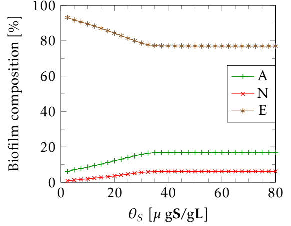
(b) Biofilm composition with respect to \theta_S
