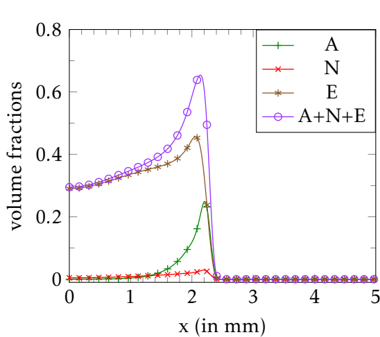
(a) Biofilm components at t = 90 days
