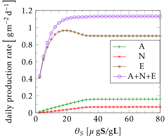
(a) Average production rate with respect to \theta_S
