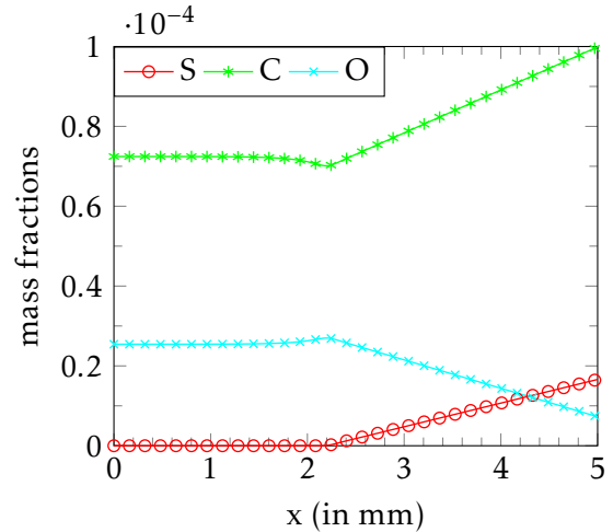
(b) Dissolved components at t = 90 days
