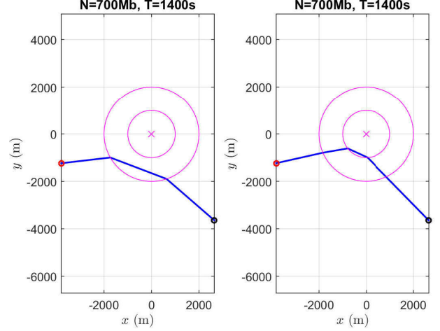
Fig. 4. The starting (resp. target) point of the vehicle is marked by a red (resp. black) point and is on the left (resp. right). The disk delineated by the pink circles correspond to geographical zones where the data rates are different. Each figure depicts, for \mathbf{u}_1^*(t) (left) and \mathbf{u}_2^*(t) (right), the vehicle trajectory which aims at uploading its data to the base station and minimizing the cost of motion to reach the target. The similarity with the refraction law in optics is well illustrated.
