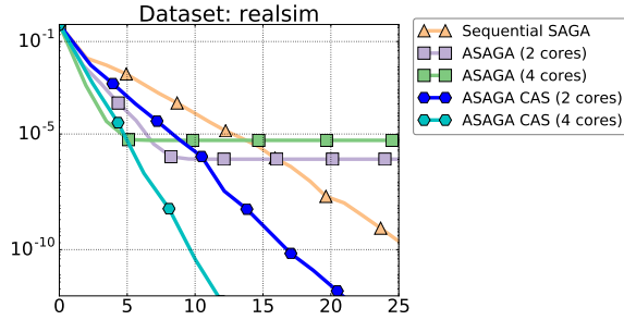
Figure 6: Compare and swap in the implementation of ASAGA. Suboptimality as a function of time for ASAGA, both using compare-and-swap (CAS) operations and using standard operations. The graph reveals that CAS is indeed needed in a practical implementation to ensure convergence to a high precision.
