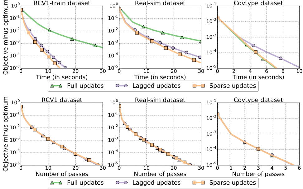
Figure 5: Lagged vs sparse SAGA updates. Suboptimality with respect to time for different SAGA update schemes on various datasets. First row: suboptimality as a function of time. Second row: suboptimality as a the number of passes over the dataset. For sparse datasets (RCV1 and Real-sim), lagged and sparse updates have a lower cost per iteration which result in faster convergence.
