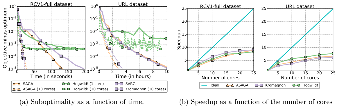
Figure 1: Convergence and speedup for asynchronous stochastic gradient descent methods. We display results for RCV1 and URL. Results for Covtype can be found in Appendix D.2.
