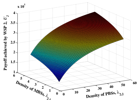
Fig. 7. The payoff achieved by WSP 2 vs. the densities of MBSs and PBSs.
