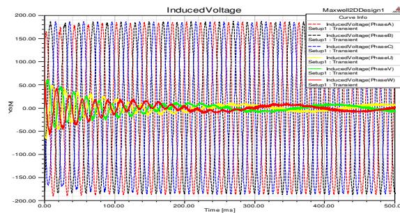
Fig. 13. DFIG stator and rotor induced voltage
