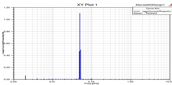
Fig. 14. DFIG stator winding current spectrum
