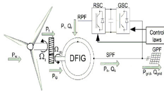
Fig. 2. Typical configuration of a DFIG wind turbine
