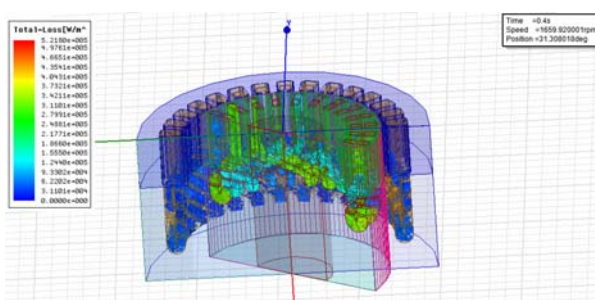
Fig. 24. 3D Total loss of DFIG inner rotor
