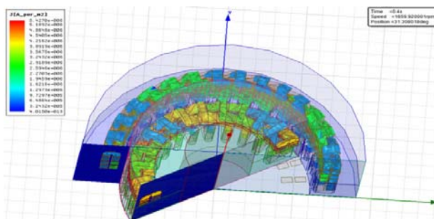
Fig. 23. 3D current density of DFIG at 0.4s
