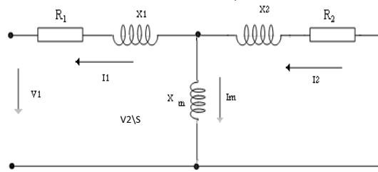
Fig. 3. DFIG equivalent circuit
