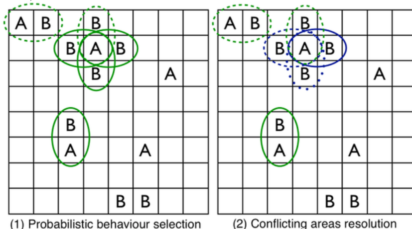
Figure 3. In (1), a behaviour can be applied several times during one simulation step. In this example the system detects that the entities A and B are in contact. The probability to perform the behaviour, if the entities are found in contact, is 0.8. So, of the six areas where the behaviour can be performed, four are kept (continuous circles) whereas two are not (dotted circle). Note that this area configuration can change accordingly to the random numbers generated. Moreover notice that three areas are in conflict and must be treated before the action can be applied (continuous circles including the same entity A). In (2), the system manage the conflicting areas. Among them, only one can be kept (the horizontal continuous circle) whereas the two others cannot. All conflicting areas have the same probability to be kept (or not kept). Note that the probabilities of behaviours have already been validated before the conflicting areas are treated. Finally, only two areas will apply the behaviour (continuous circles)
