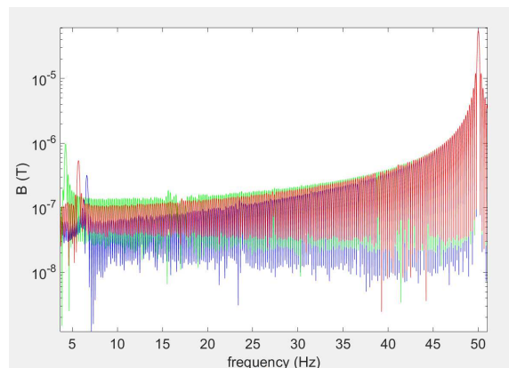
Fig.19 Dynamic eccentricity typical frequency for three different motors
