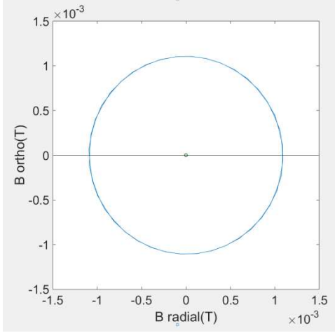
Fig.5 Lissajou of stray rotating field for an equilibrate and unfaulty machine in simulation
