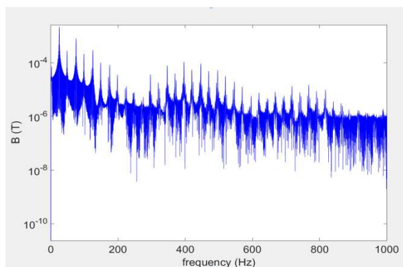
Fig.4 Spectrum of stray field with faults in simulation
