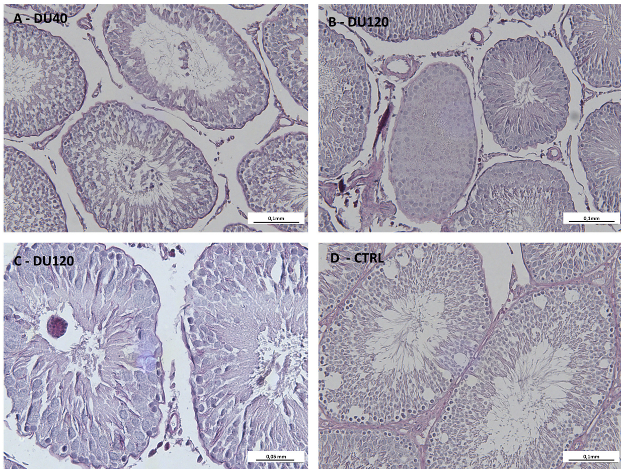
Fig. 1. Effects of DU exposure on testis histology. All stages of seminiferous epithelium appeared normal, and only occasional abnormalities were observed as germ cell sloughing (s), tubules without lumen (l), multinucleated giant cells (m). Basal vacuoles were observed in the CTRL group and the number of seminiferous tubules with vacuoles decreased in both DU groups. Corresponding bars are indicated in each figure.
