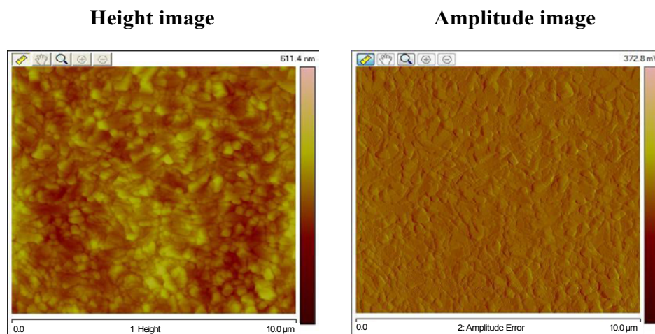
Figure 6: Height and amplitude images (10 \mu\text{m} *10 \mu\text{m} ) obtained in AFM with the tapping mode for surfaces functionalized with a mixture of NPs + (PAH-PSS) 3 -PAH.
