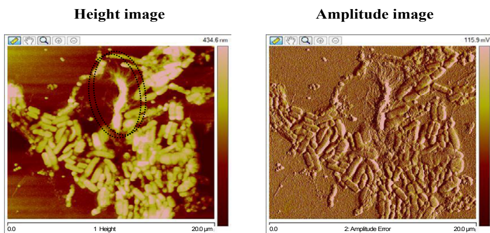
Figure 7: Height and amplitude images (20 \mu\text{m} *20 \mu\text{m} ) obtained in AFM with the tapping mode for surfaces modified with a mixture of NPs and bacteria.
