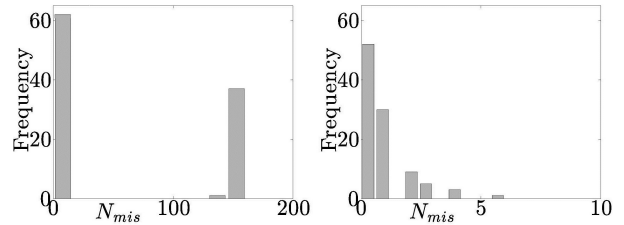
Fig. 2. Distributions of the number of mislabelled pixels N_{\text{mis}} before using SA (left) and after using SA (right).
