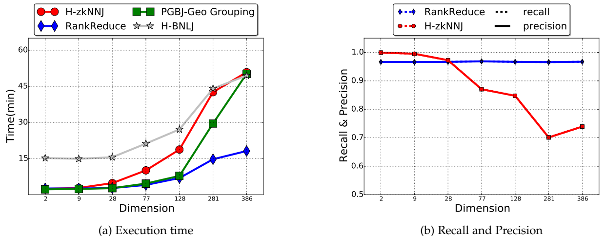
Fig. 13: Generated datasets of various dimensions
