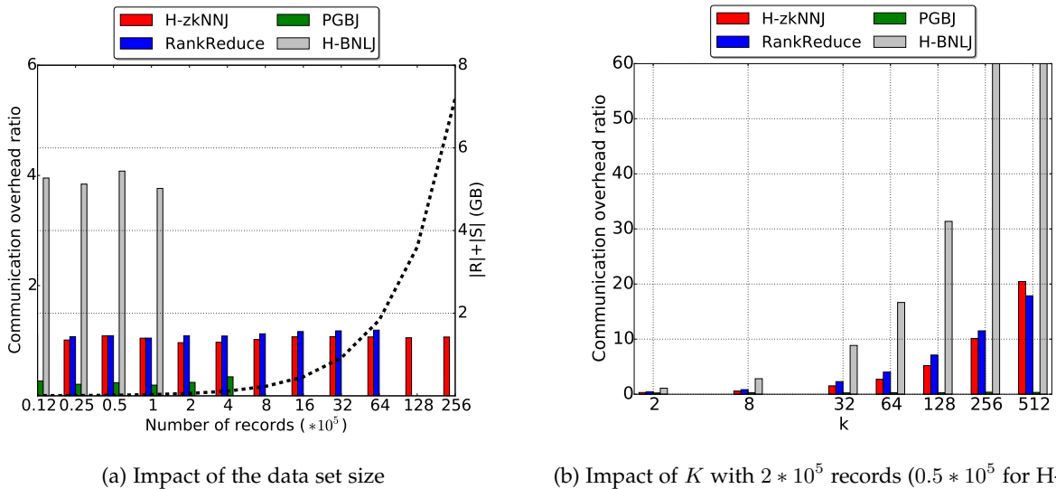
Fig. 8: Geo dataset, communication overhead
