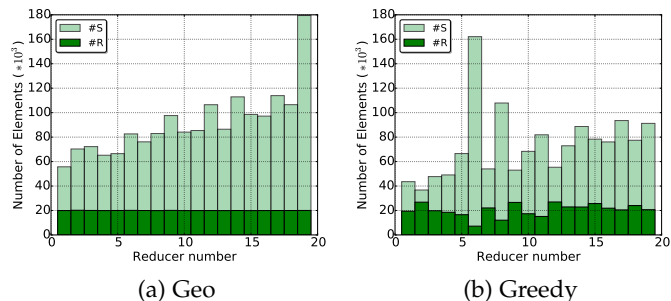
Fig. 16: PGBJ, load balancing with 20 reducers
