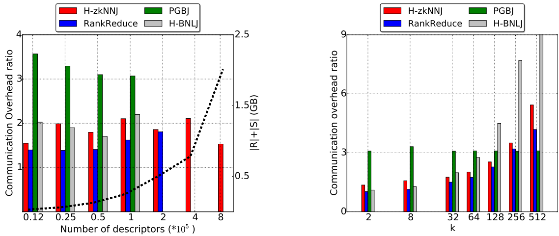
(a) Surf, impact of the dataset size
