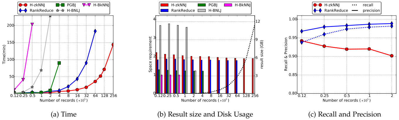
Fig. 6: Geo dataset impact of the data set size
