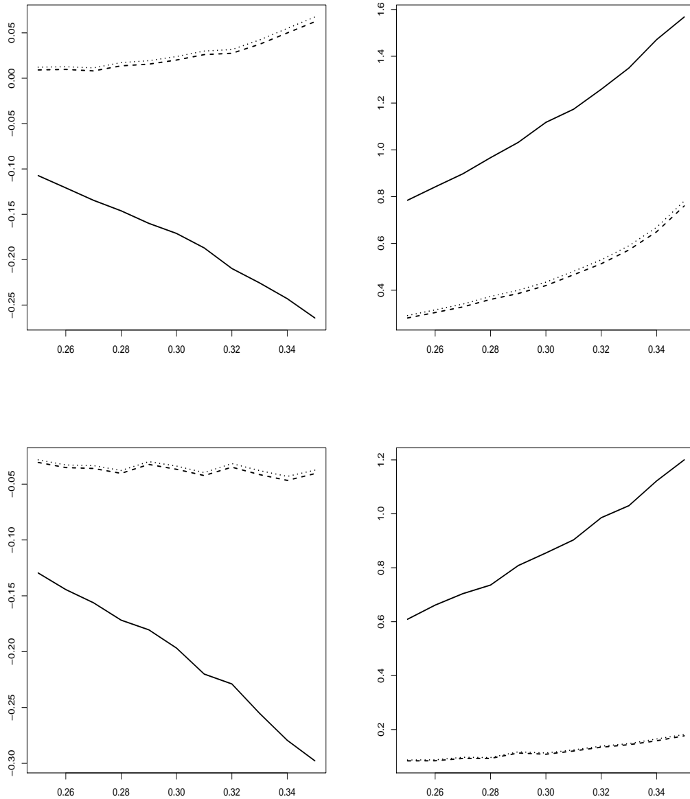
Figure 4: Extreme PH(1/2) estimation with \delta = 0.999 , for \gamma \in [0.25, 0.35] . Left panels: non-conditioned cases, right panels: conditioned cases. Top: Case of the Fréchet distribution, bottom: case of the Burr distribution with \rho = -5 . Full line: PL estimator, dotted line: CTrim-PL estimator, dashed line: CWins-PL estimator.
