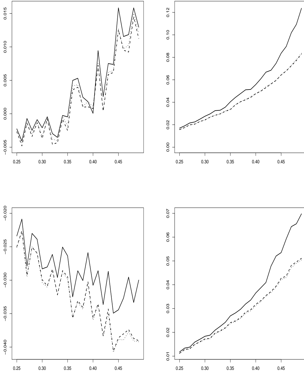
Figure 1: Extreme TVaR estimation with \delta = 0.999 , for \gamma \in [0.25, 0.49] . Left panels: relative bias, right panels: relative MSE. Top: Case of the Fréchet distribution, bottom: case of the Burr distribution with \rho = -5 . Full line: PL estimator, dotted line: CTrim-PL estimator, dashed line: CWins-PL estimator.
