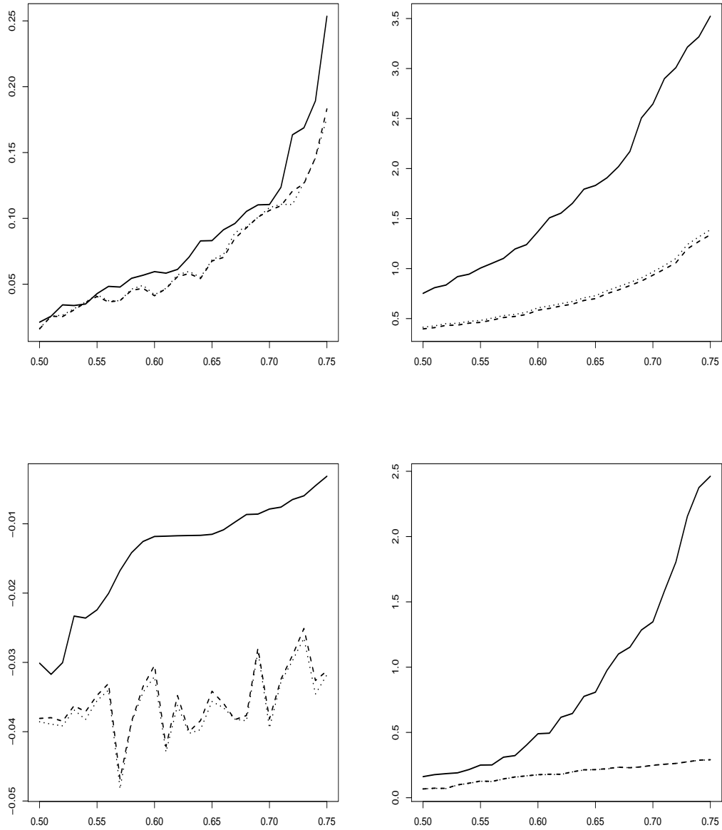
Figure 3: Extreme TVaR estimation with \delta = 0.999 , for \gamma \in [0.5, 0.75] . Left panels: non-conditioned cases, right panels: conditioned cases. Top: Case of the Fréchet distribution, bottom: case of the Burr distribution with \rho = -5 . Full line: PL estimator, dotted line: CTrim-PL estimator, dashed line: CWins-PL estimator.
