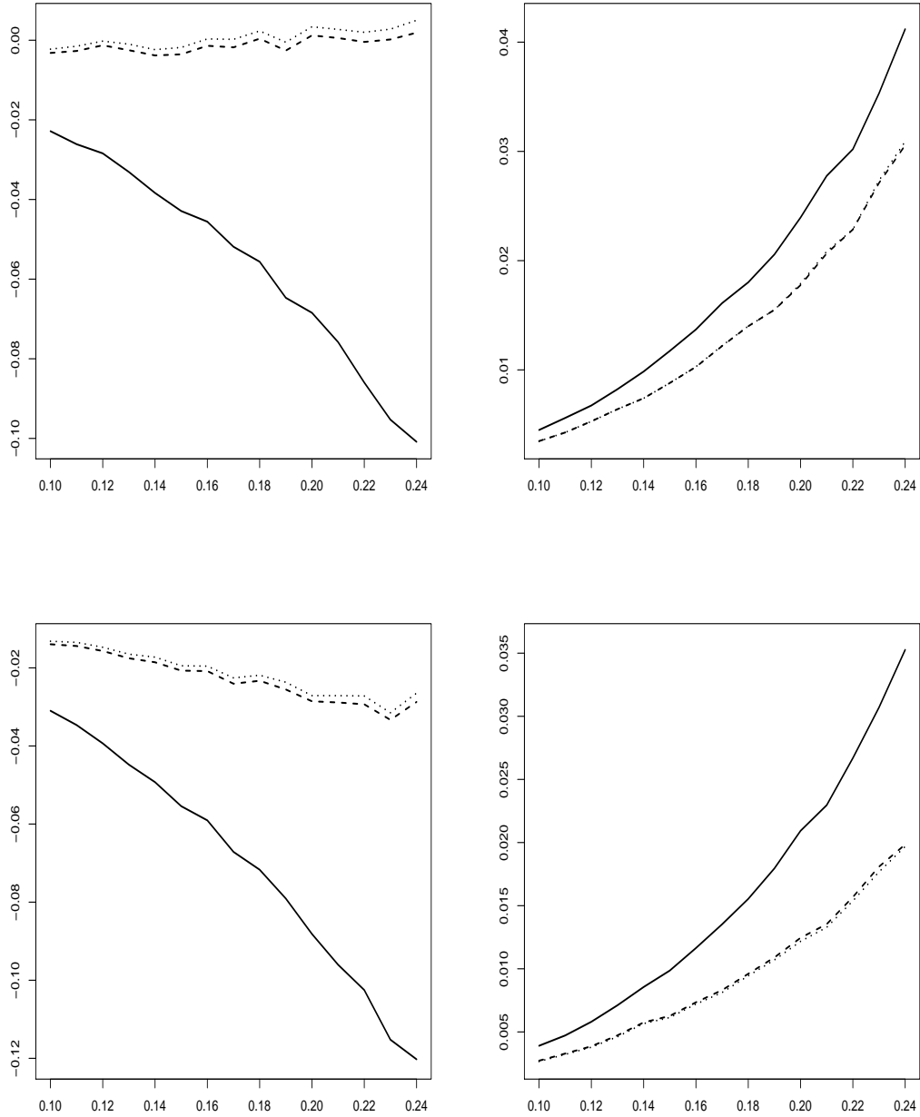
Figure 2: Extreme PH(1/2) estimation with \delta = 0.999 , for \gamma \in [0.1, 0.24] . Left panels: relative bias, right panels: relative MSE. Top: Case of the Fréchet distribution, bottom: case of the Burr distribution with \rho = -5 . Full line: PL estimator, dotted line: CTrim-PL estimator, dashed line: CWins-PL estimator.
