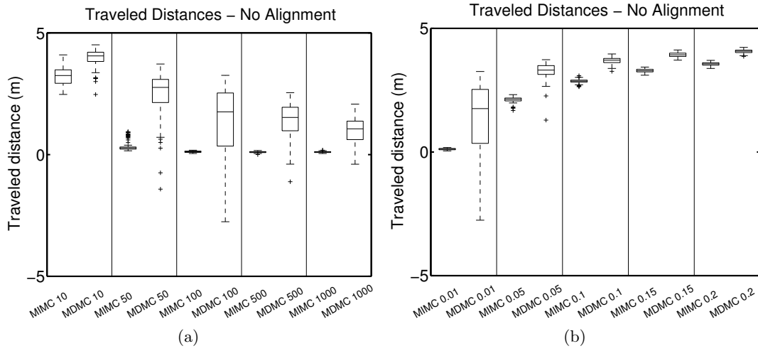
Figure 8: MDMC vs MIMC in simulations with informed robots and no alignment control. Box-plots of the distribution of effective traveled distance for (a) different swarm sizes ( \rho = 0.01 ) and (b) different proportions of informed robots ( N = 100 ).
