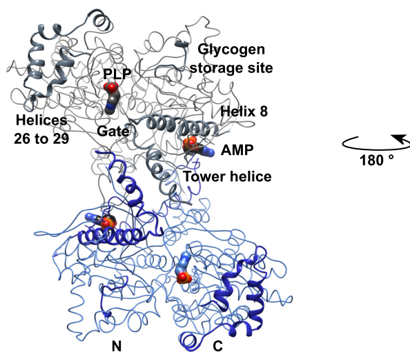
FIGURE 2. Overview of the structure of AMP-bound brain glycogen phosphorylase. Shown are schematic and ribbon representations of the C_{\alpha} trace of the tetramer and functional dimer of bGP. Key secondary structures described in this study are indicated. The catalytic site and the AMP-binding site are marked by the co-factor pyridoxal phosphate and allosteric effector AMP (surface representation), respectively. a , the tetrameric organization of bGP. Two bGP monomers associate by the horizontal axis to form the functional dimer (monomers 1 and 2). The tetramer is composed of two functional dimers that interact through their catalytic faces, by the vertical axis . The association of two monomers through the catalytic site forms the packing dimer (monomers 1 and 3). A schematic representation of the tetramer is shown ( right panel ). The functional dimer corresponds to the association of monomers 1 and 2 ( gray and blue ) and monomers 3 and 4 ( turquoise and purple ). The packing dimer corresponds to the association of monomers 1 and 3 ( gray and turquoise ) and monomers 2 and 4 ( blue and purple ). b , the catalytic face of bGP. The residues implied in the activation of GP and the subunit interfaces are indicated. The gate loop (residues 279–289) is not stabilized allowing the glycogen to access the catalytic site. The tower helix interacts with its counterparts from the other subunits. The crossover angle of the tower helices in the functional dimer avoids the stabilization of the gate, promoting the opening of the catalytic site. c , the regulatory face of bGP contains key regions involved in the control of allosteric transition of the enzyme and is exposed to solvent in both the tetramer and the dimer. PLP , pyridoxal phosphate.
