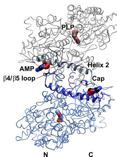
FIGURE 2. Overview of the structure of AMP-bound brain glycogen phosphorylase. Shown are schematic and ribbon representations of the C_{\alpha} trace of the tetramer and functional dimer of bGP. Key secondary structures described in this study are indicated. The catalytic site and the AMP-binding site are marked by the co-factor pyridoxal phosphate and allosteric effector AMP (surface representation), respectively. a , the tetrameric organization of bGP. Two bGP monomers associate by the horizontal axis to form the functional dimer (monomers 1 and 2). The tetramer is composed of two functional dimers that interact through their catalytic faces, by the vertical axis . The association of two monomers through the catalytic site forms the packing dimer (monomers 1 and 3). A schematic representation of the tetramer is shown ( right panel ). The functional dimer corresponds to the association of monomers 1 and 2 ( gray and blue ) and monomers 3 and 4 ( turquoise and purple ). The packing dimer corresponds to the association of monomers 1 and 3 ( gray and turquoise ) and monomers 2 and 4 ( blue and purple ). b , the catalytic face of bGP. The residues implied in the activation of GP and the subunit interfaces are indicated. The gate loop (residues 279–289) is not stabilized allowing the glycogen to access the catalytic site. The tower helix interacts with its counterparts from the other subunits. The crossover angle of the tower helices in the functional dimer avoids the stabilization of the gate, promoting the opening of the catalytic site. c , the regulatory face of bGP contains key regions involved in the control of allosteric transition of the enzyme and is exposed to solvent in both the tetramer and the dimer. PLP , pyridoxal phosphate.
