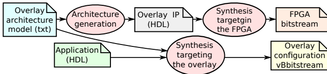
Fig. 1. Two flows: overlay synthesis on the FPGA, and application synthesis on the overlay.
