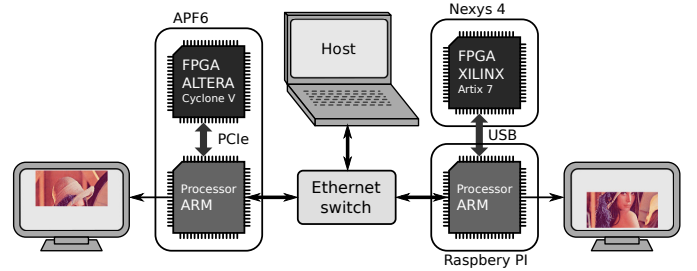
Fig. 2. Experimental setup.
