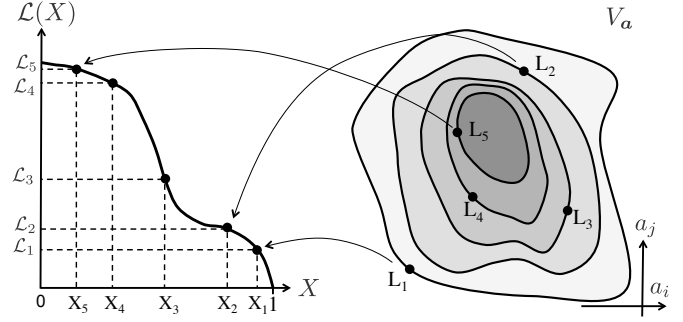
Figure 1: Visualisation of the integral of \mathcal{L}(X) and corresponding volumes on the parameter space (two parameters only, a_i, a_j are considered with a 2D representation).
