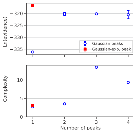
Figure 10: Evidence and complexity of the different considered models.
