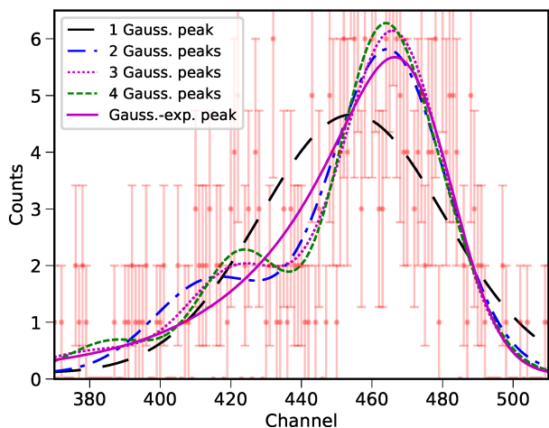
Figure 9: Profile curves corresponding to the likelihood maxima of the different models (1–4 Gaussian peaks and Gaussian-exponential peak).
