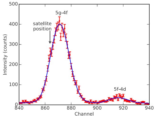
Figure 8: Pionic nitrogen 5 – 4 transitions. Possible additional transitions from the presence of one remaining electron in the K shell are indicated
