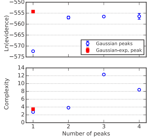
Figure 10: Evidence and complexity of the different considered models.
