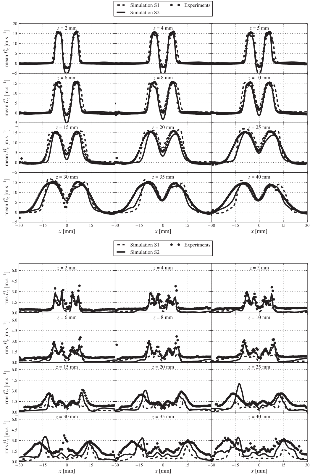
Fig. 13. 1-D radial profiles of the axial velocity U_z at different distances z from the bluff-body wall surface for the case X_{\text{H}_2}^{\text{fuel}} = 0.60 . (top) Mean profiles. (bottom) RMS profiles.
