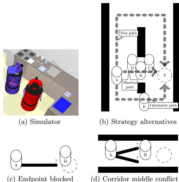
Figure 1: (a) Experiments with 2 robots in Gazebo Simulator. (b) Strategy alternatives: Collision free path, shortest path ignoring humans, optimistic path balancing length vs. human comfort. (c) Conflict for goal location. (d) Conflict to find path to goal.
