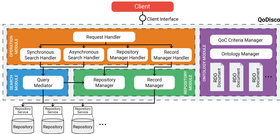
Fig. 1. QoDisco architecture
